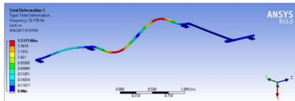
Gambar. 3. Mode Shape #3 Support #1
