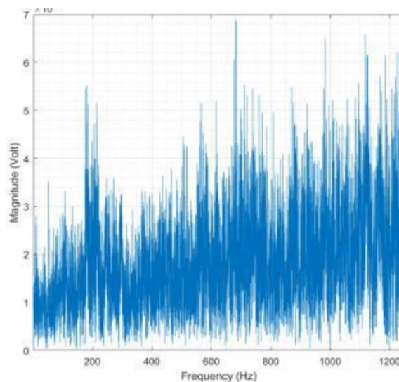
Gambar 6. Spektrum 1 Radial Support 1
