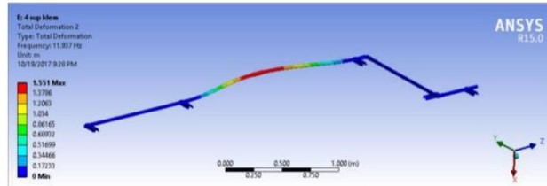
Gambar. 2. Mode Shape #2 Support #1
