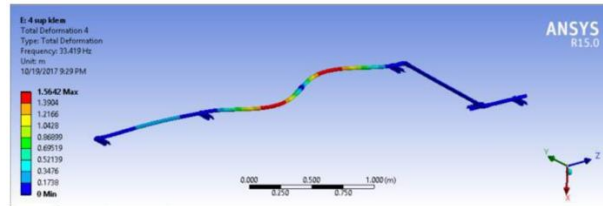
Gambar. 4. Mode Shape #4 Support #1
