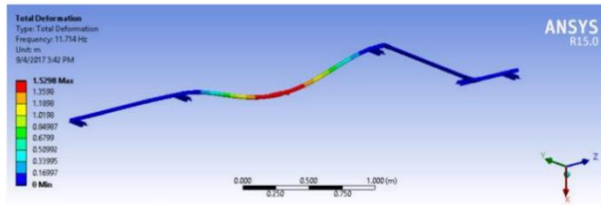
Gambar. 1. Mode Shape #2 Support #1
